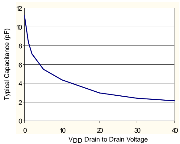
Figure 8. Typical Output Capacitance
